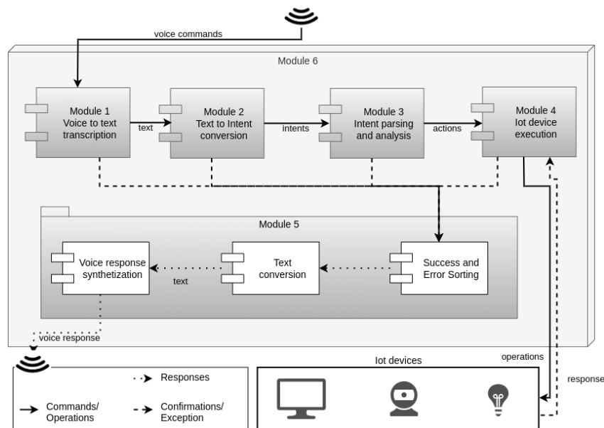
Figure 2. A.D.A. Architecture
